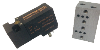
Midi POPET VALF N.A. POPPET VALVE ( midi ) 24 v dc 3/2 N.O.
